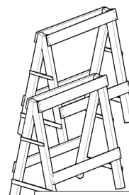
SAWHORSES
